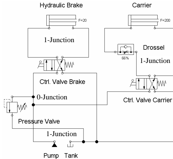
Figure 3. Hydraulic installation under fault diagnosis.
