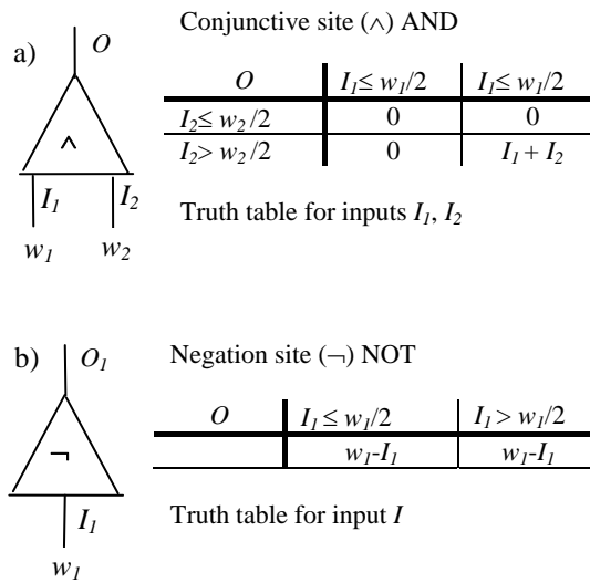
Figure 1. Neural sites for logical aggregation of effects to causes.
